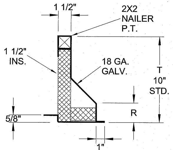
RPC-1D SECTION
