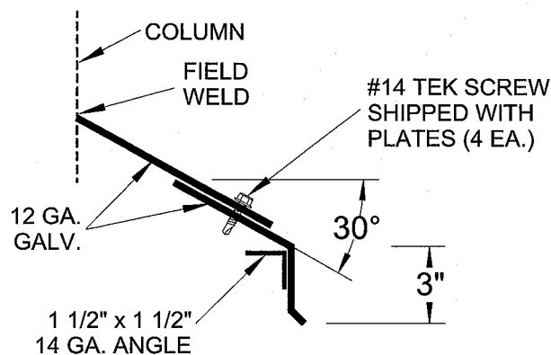
SECTION A
