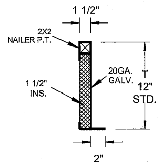
RPEJ-3 SECTION
