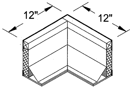
ISOMETRIC VIEW RPEJ-2 INSIDE CORNER
