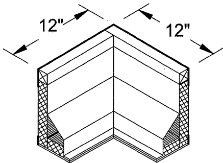
ISOMETRIC VIEW RPEJ-1 INSIDE CORNER
