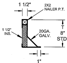
RPEJ-2 SECTION
