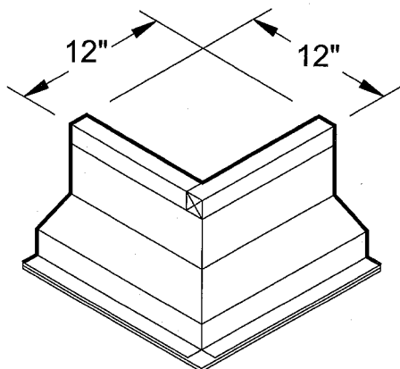
ISOMETRIC VIEW RPEJ-1 OUTSIDE CORNER
