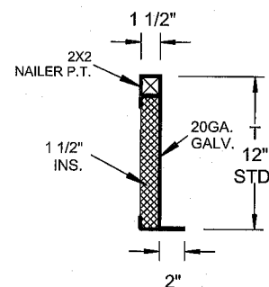
RPEJ-3 SECTION
