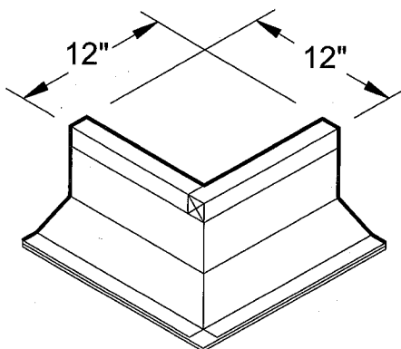
ISOMETRIC VIEW RPEJ-2 OUTSIDE CORNER
