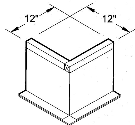
ISOMETRIC VIEW RPEJ-3 OUTSIDE CORNER
