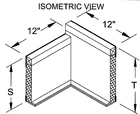
RPEJ-3 LEFT INSIDE CORNER (L.I.C.)
