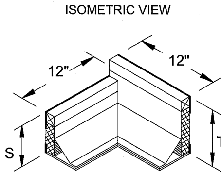
RPEJ-2 LEFT INSIDE CORNER (L.I.C.)
