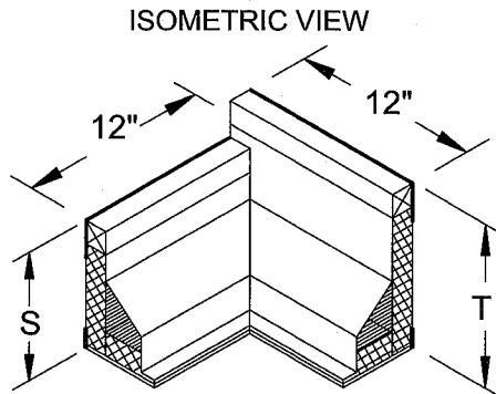
RPEJ-1 LEFT INSIDE CORNER (L.I.C.)
