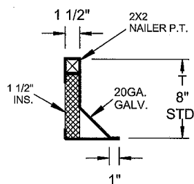
RPEJ-2 SECTION
