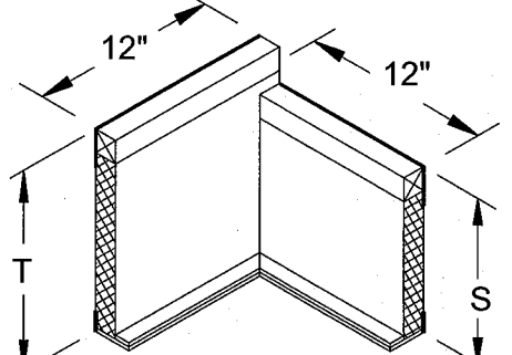
RPEJ-3 RIGHT INSIDE CORNER (R.I.C.)
