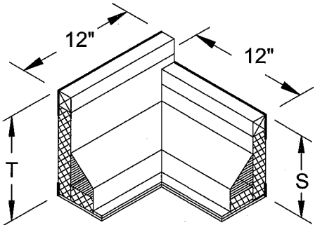
RPEJ-1 RIGHT INSIDE CORNER (R.I.C.)
