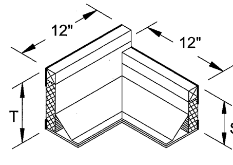
RPEJ-2 RIGHT INSIDE CORNER (R.I.C.)
