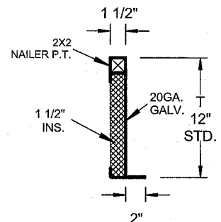
RPEJ-3 SECTION
