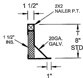
RPEJ-2 SECTION
