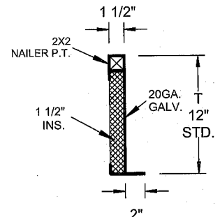
RPEJ-3 SECTION
