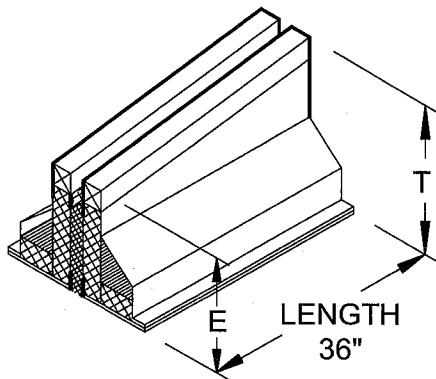
ISOMETRIC VIEW RPEJ-1 SLOPED ENDS
