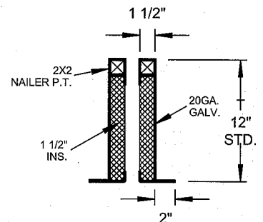
RPEJ-3 SECTIONS
