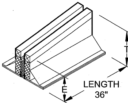
ISOMETRIC VIEW RPEJ-2 SLOPED ENDS
