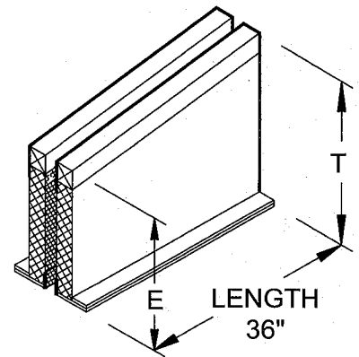
ISOMETRIC VIEW RPEJ-3 SLOPED ENDS
