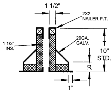
RPEJ-1 SECTIONS
