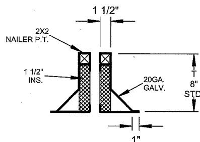
RPEJ-2 SECTIONS
