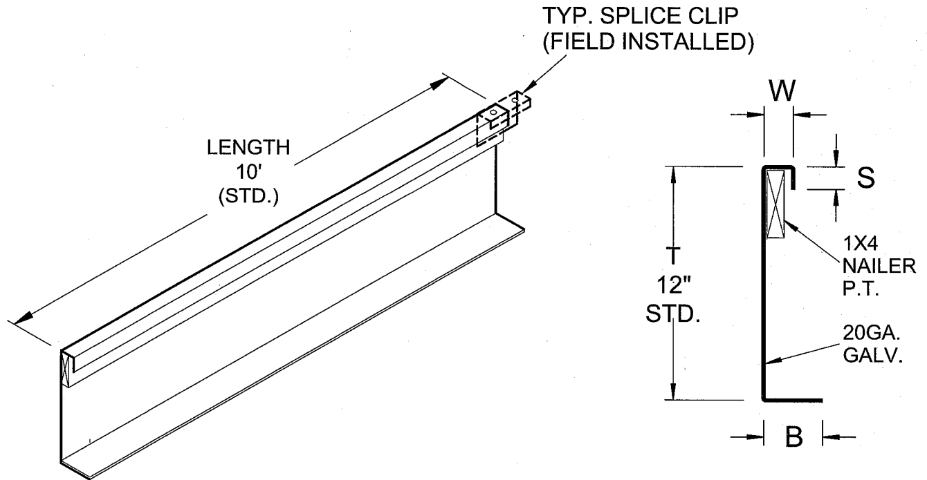
ISOMETRIC VIEW
